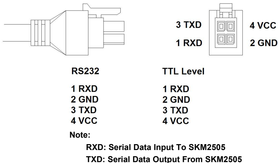
图 2: SKM3507MR-40MXT 接口定义/Interface definition
