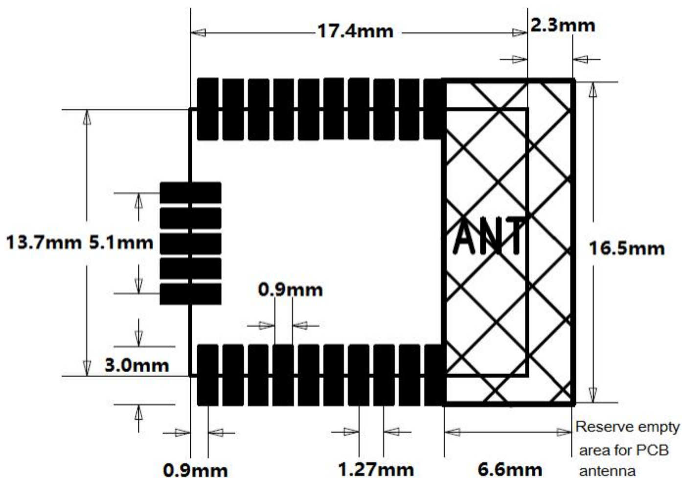
Figure 8 推荐 PCB 封装/ SKB380 Recommended PCB Footprint
