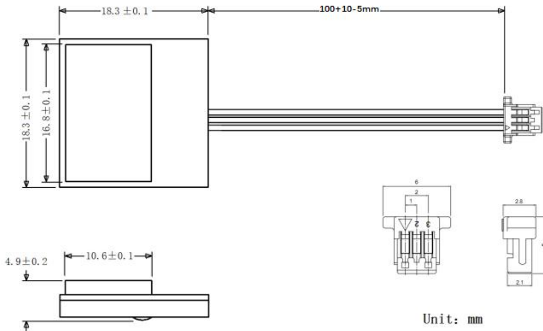
Figure 3: SKM81DC Dimensions
